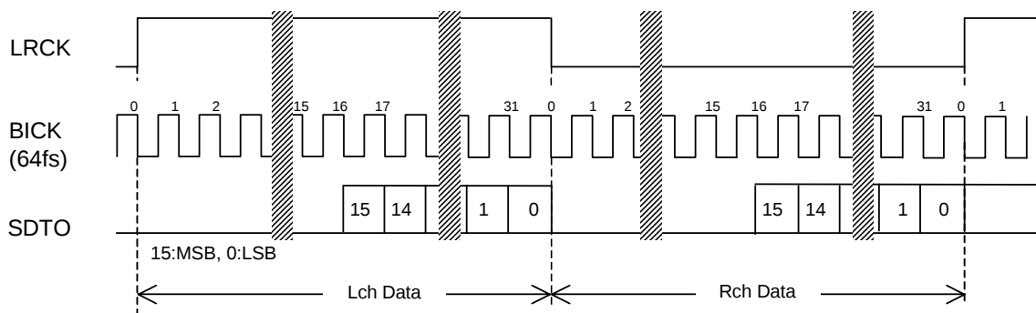
Figure 21. Mode 0 Timing
