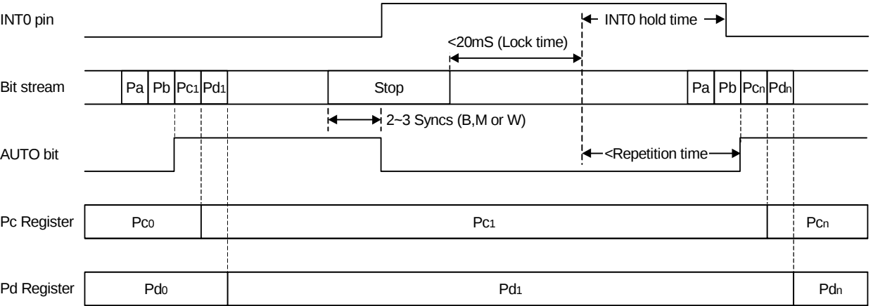
Figure 28. Timing example 2
