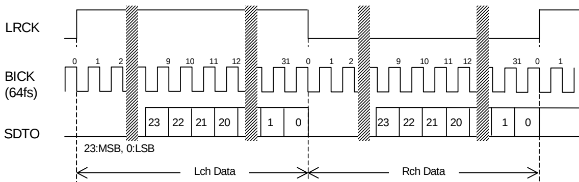
Figure 22. Mode 3 Timing
