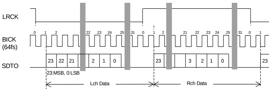
Figure 24. Mode 5 Timing
