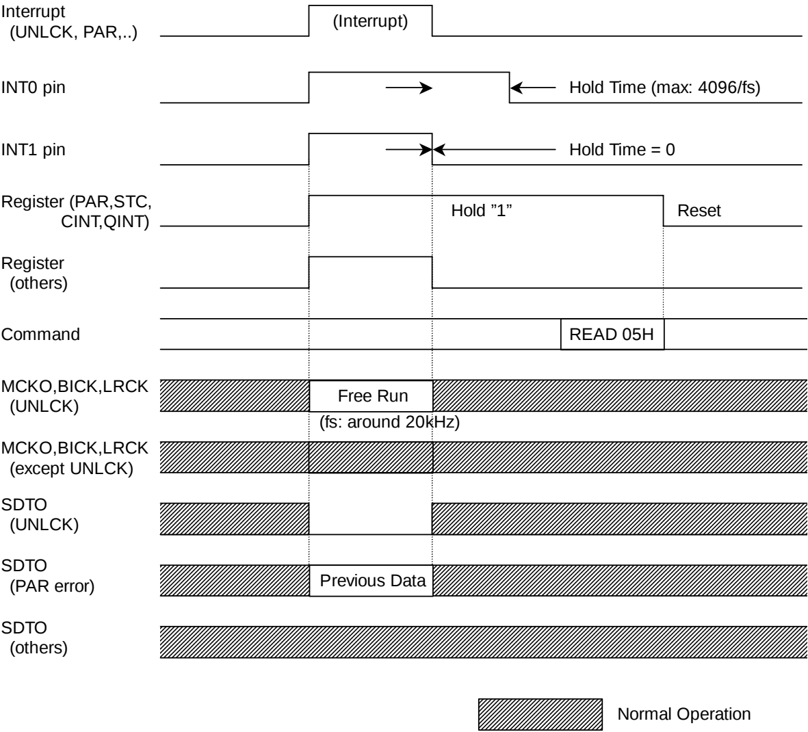
Figure 17. INT1-0 pin timing
