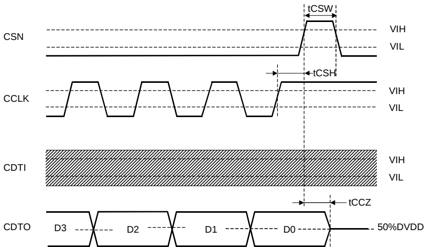
Figure 6. READ Data Input Timing 2
