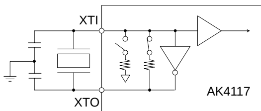
Figure 8. X'tal mode (EXCK= "0")
