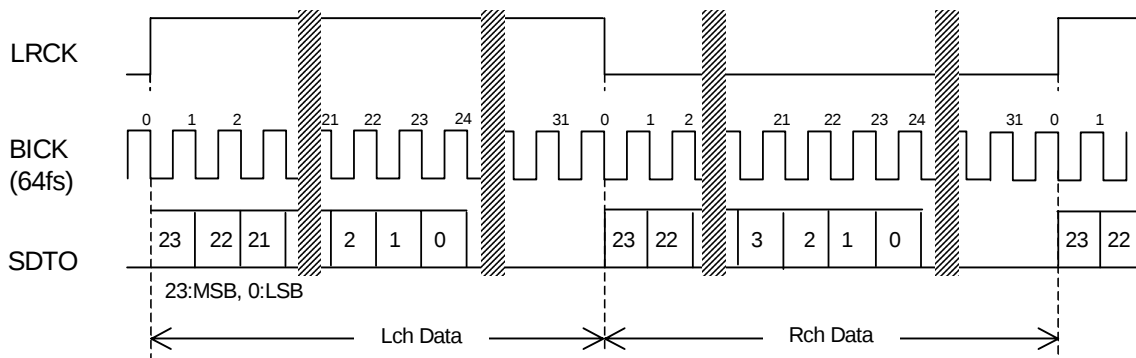
Figure 23. Mode 4 Timing
